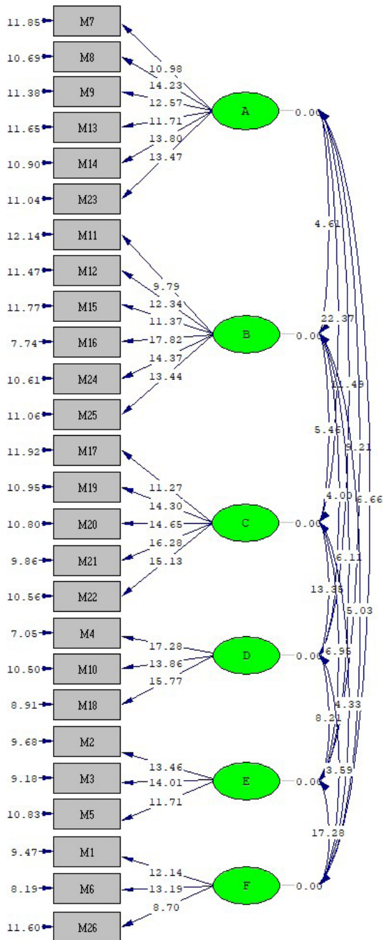
Figure 1. Path Diagram (t values)
